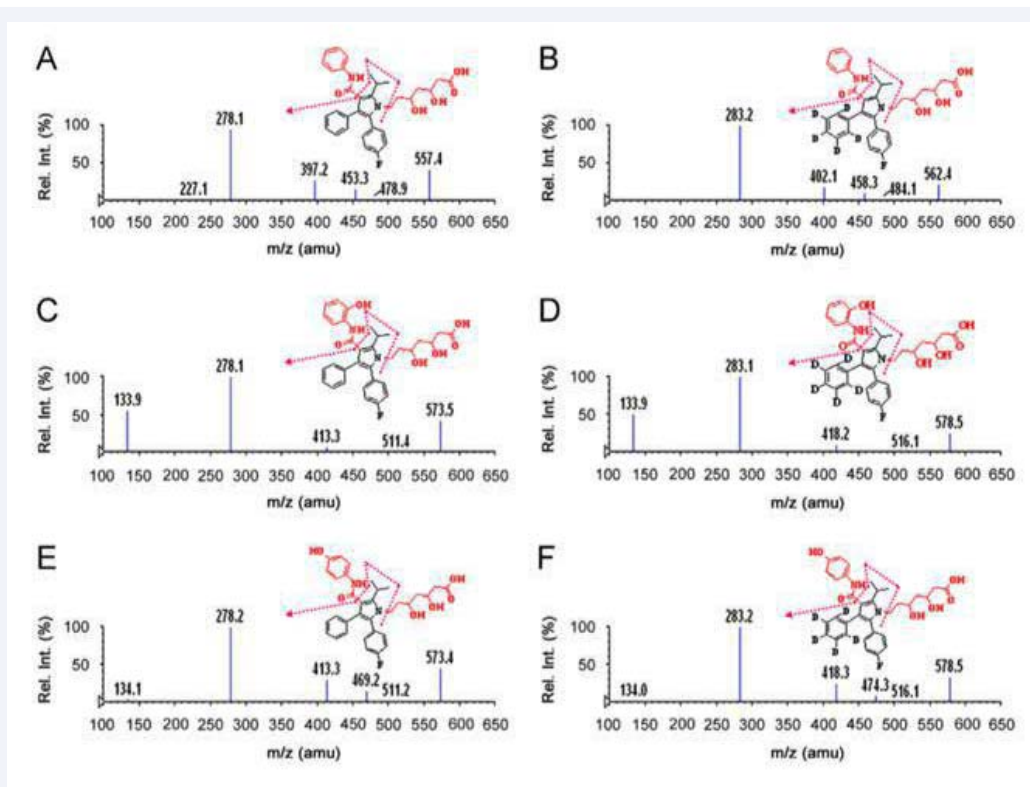
Figure 6 LC-ESI-MS spectra of ATOR compounds with negative electro spray ionization mode. The product ion spectra of (A) ATOR, (B) ATOR-D5, (C) orto-(OH-ATOR, (D) orto-OH-ATOR-D5, (E) para-(OH-ATOR, and (F) para-OH-ATOR-D5 [107].
