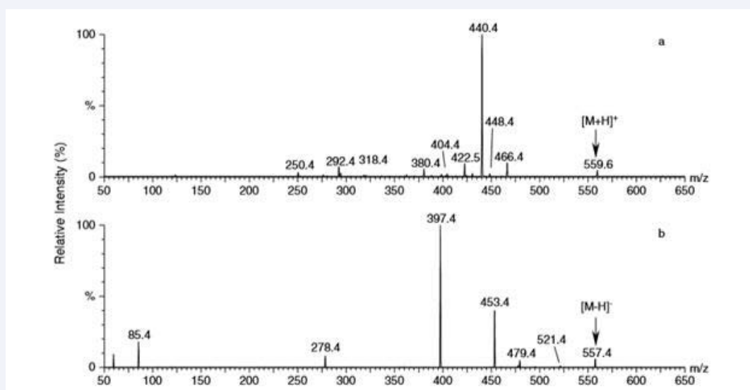
Figure 11 Mass spectra of atorvastatin. (a) [M+H]^+ and (b) [M-H]^- . The ion species subjected to CI is indicated with a vertical arrow. The applied laboratory collision energies were (a) 24 and (b) 26 eV [119].
