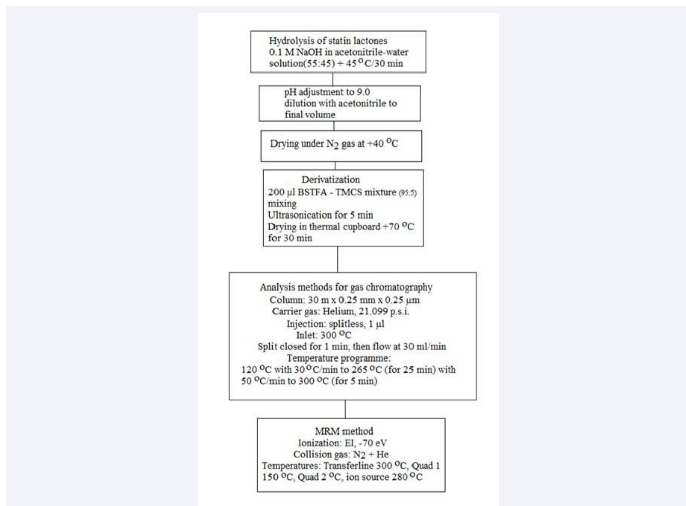
Figure 13 Scheme of the experimental procedures used to study statins from wood hydrolysis with fungi microbes. Separation (incl. ATOR) analysis made with GC-MRM-MS/MS after silylation of statins [42].
