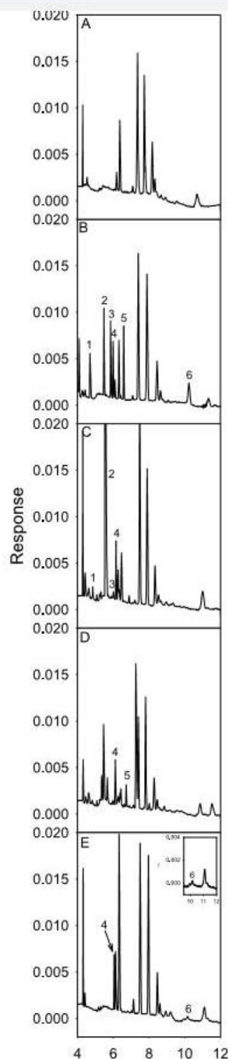
Figure 17 Electropherograms of the separation of drugs in biological samples. (A) plasma blank; (B) plasma spiked 100 ng/mL for AM and DO, 200 ng/mL for ATOR, IR, and RO with 200 ng/mL IS; (C) plasma sample from a patient receiving 5 mg of AM (Norvasc R) orally, 5 mg of DO (Aricept R), and 150 mg of IR (Aprovel R); (D) plasma from a patient receiving 40 mg of ATOR (Lipitor R) orally at steady state; (E) oral administration of 20 mg RO (Crestor R) with single dosing after healthy volunteer plasma. Peaks: 1, amiloride; 2, irbesartan; 3, donepezil; 4, IS diclofenac; 5, atorvastatin; 6, rosuvastatin [149].
