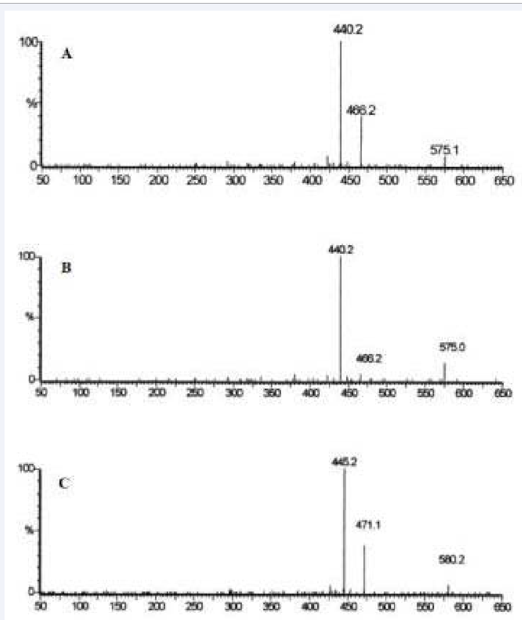
Figure 8 Mass fragmentation spectra of ATOR metabolites and the deuterated analogue of ortho- hydroxyl metabolite. Electrospray product ion mass spectra of ortho-hydroxyl ATOR ( [M+H]^+ 575.3 Da) (A), and para-hydroxyl ATOR ( [M+H]^+ 575.3 Da) (B), and [D_5] -ortho-hydroxyl ATOR ( [M+H]^+ 580.3 Da) (C) [109].
