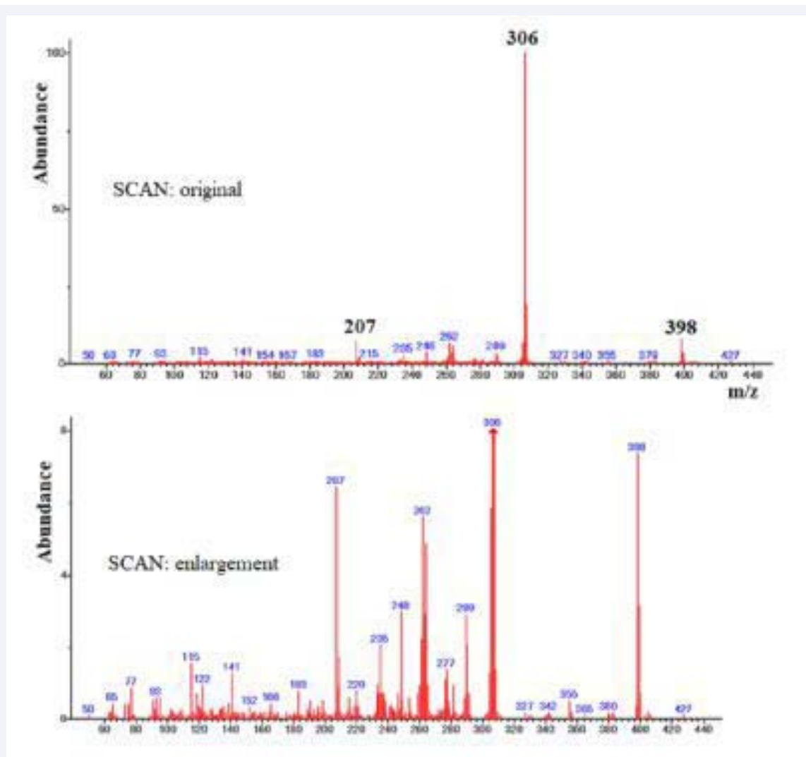
Figure 15 ATOR-TMS (EI Scan 28.298-28.278 min, 11 scans). Silylated ATOR-A has m/z 631.3 Da (exact mass 558.2530 Da, trimethyl silyl group 73 Da). The fragmentation could not be detected at higher abundance than 10%. Therefore, the m/z below 450 Da were used [141].
