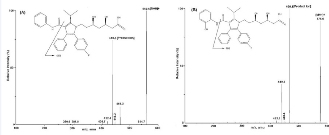
Figure 5 Mass spectra from LC-MS analyses. Full scan positive ions spray ionization. Product ion mass spectra and the proposed patterns of fragmentation of (A) atorvastatin and (B) ortho-hydroxy atorvastatin.
