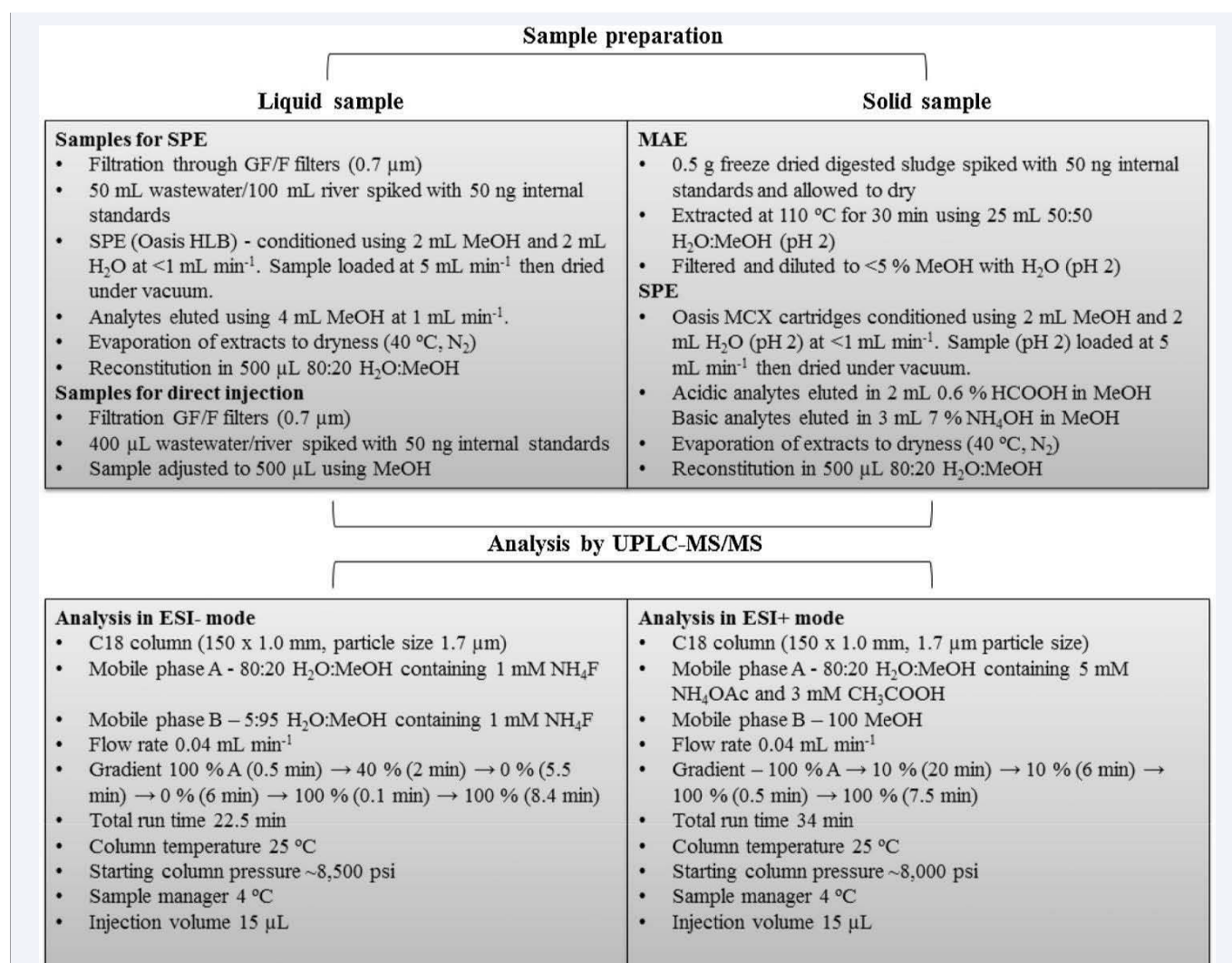
Figure 12 Overview of analytical protocol used to determine target ECs in crude wastewater, final effluent, river water and digested sludge [125].
