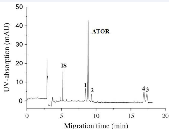
Figure 16 Optimized MEKC separation of atorvastatin and drug-related substances. Peaks: Ipravastatin; 1 desfluoro atorvastatin, ATOR = atorvastatin, 2 = diastereomer of atorvastatin, 3 = atorvastatin methyl ester and 4 = atorvastatin lactone. Separation conditions: 10 mM borate buffer, pH 9.5, 50 mM SDS, 20% (v/v) methanol, voltage 30 kV, 25 °C, detection wavelength 214 nm, hydrodynamic injection 50 mbar, 4 seconds [95].
