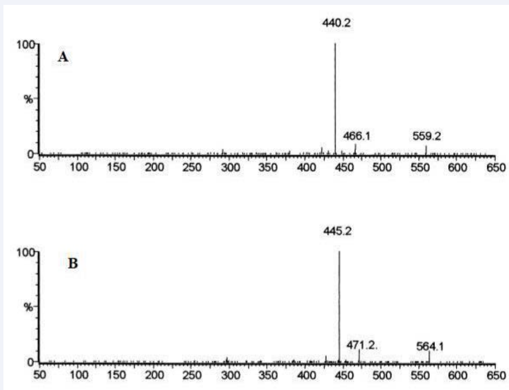
Figure 7 Mass fragmentation spectra of ATOR and its deuterated analogue. Positive electro spray ionization mode. Electro spray product ion mass spectra of the precursor ions of (A) ATOR ( [M+H]^+ m/z of 559.2 Da and (B) of [D_5] -ATOR ( [M+H]^+ m/z of 564.1 Da [109].
